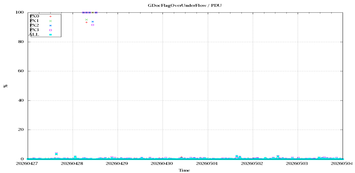
Figure 4: OverUnderFlowFlag timeseries
