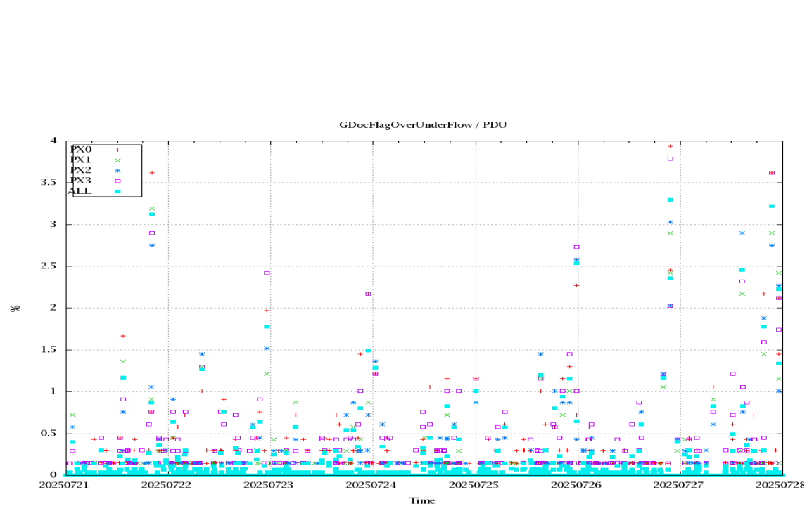
Figure 4: OverUnderFlowFlag timeseries
