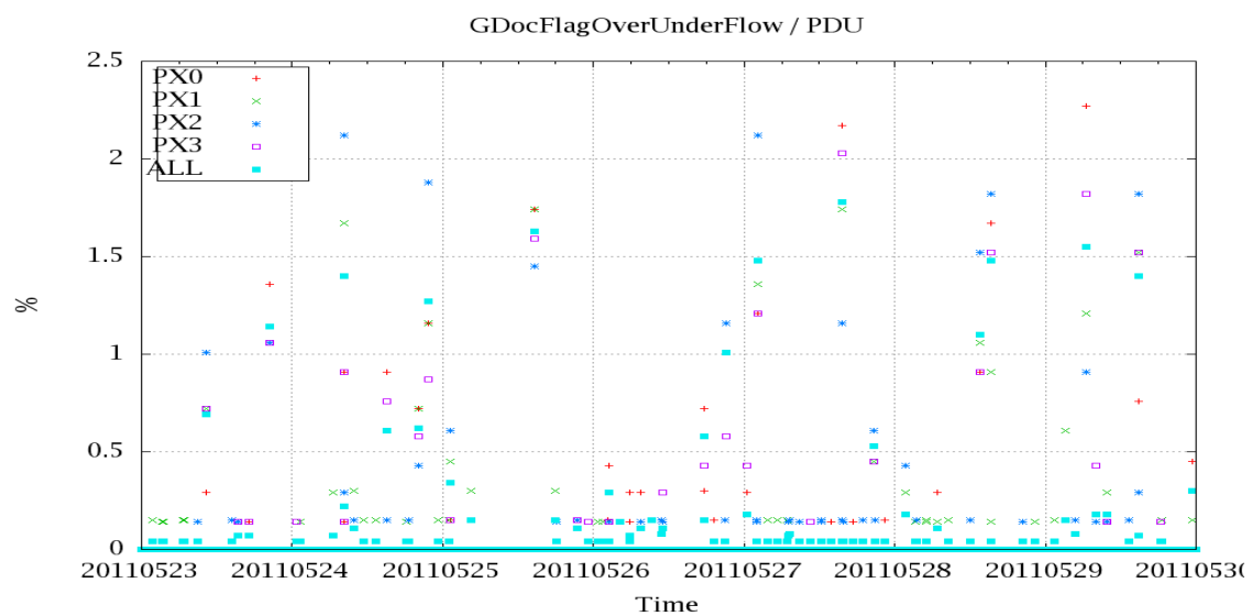
Figure 4: OverUnderFlowFlag timeseries
