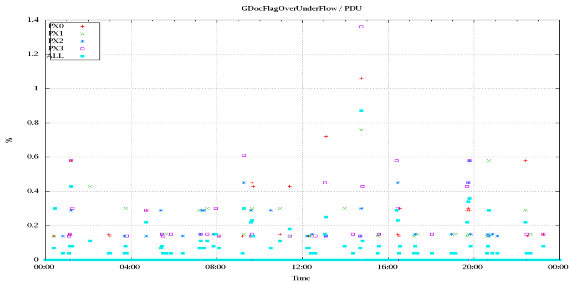
Figure 5: OverUnderFlowFlag timeseries
