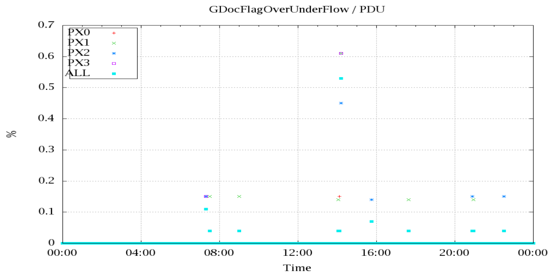
Figure 5: OverUnderFlowFlag timeseries
