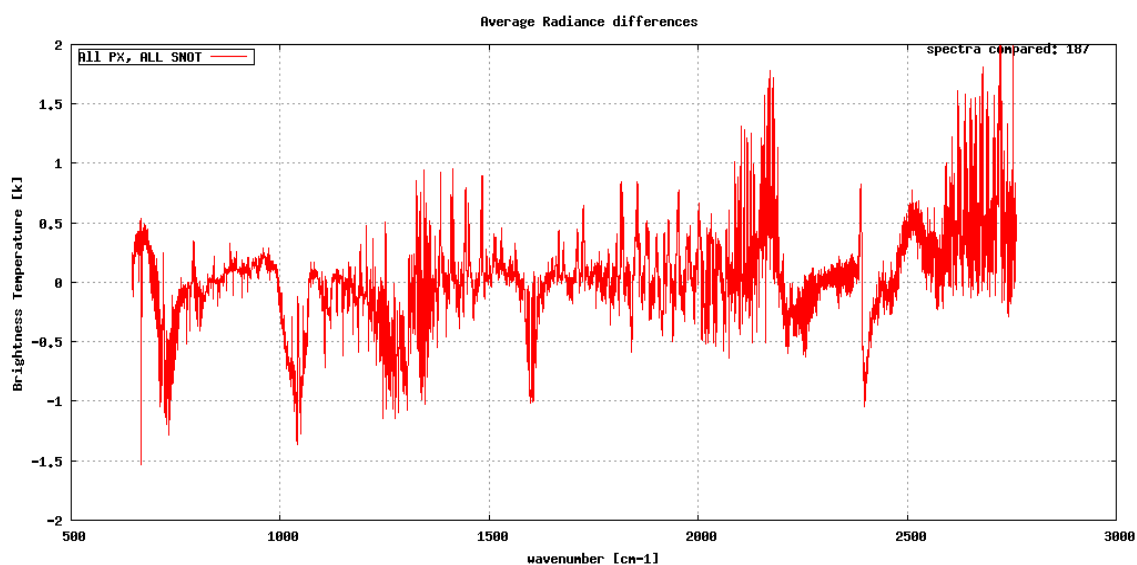
Figure 6: Average Radiance differences: IASI-RTIASI
