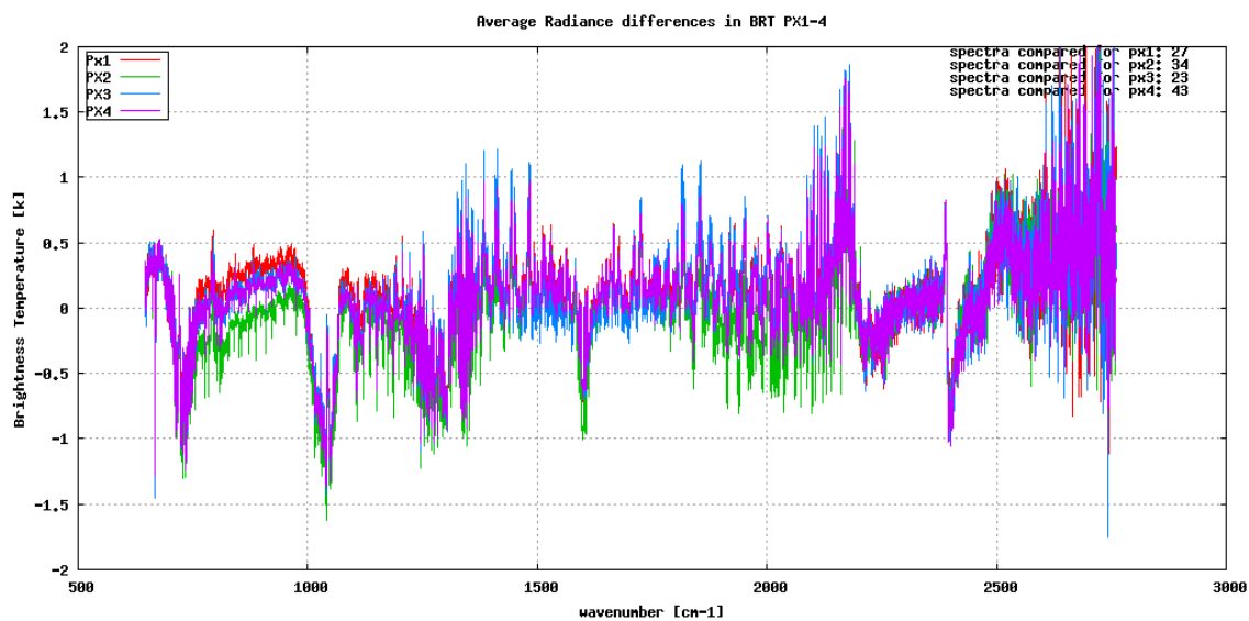
Figure 8: Average Radiance differences: IASI-RTIASI
