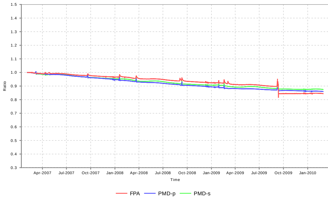
Instrument throughput (WLS) @550nm
