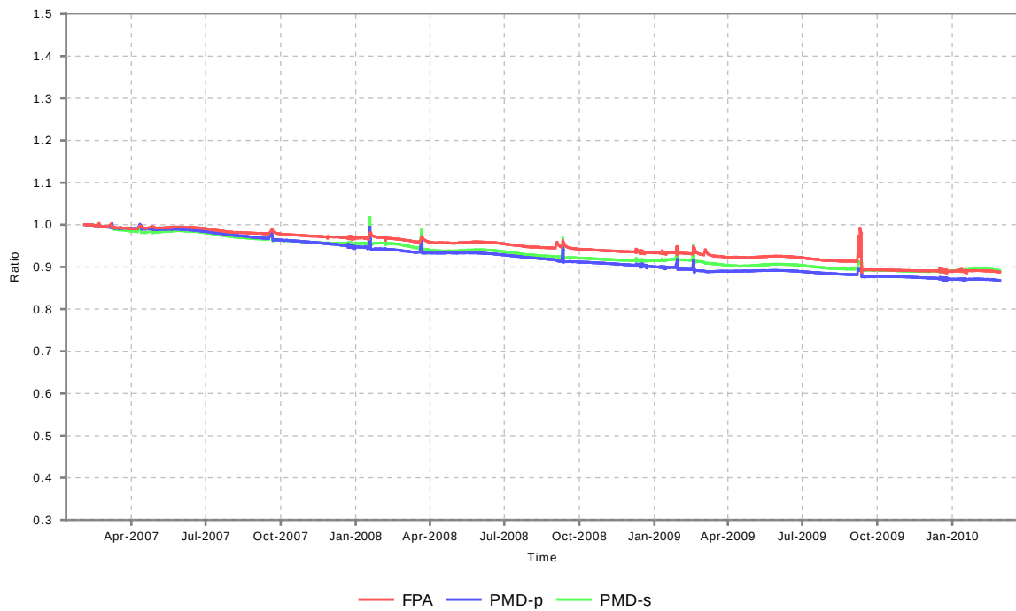
Instrument throughput (WLS) @650nm
