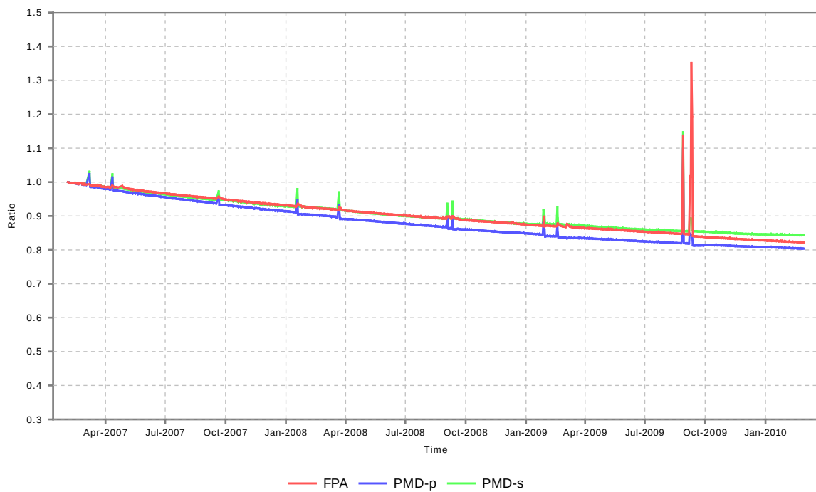
Instrument throughput (WLS) @745nm
